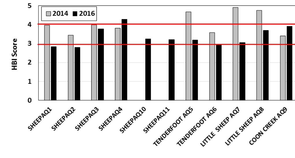
Figure 7. Macroinvertebrate HBI scores across Tintina Study Sites by year. Red lines bracket the slight organic impairment range (3.0-4.0), below 3.0 indicates minimal impairment.
